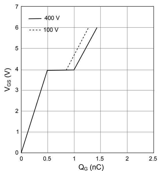
Figure 22. Typical Gate Charge (HS) at T_J=25^\circ\text{C}
