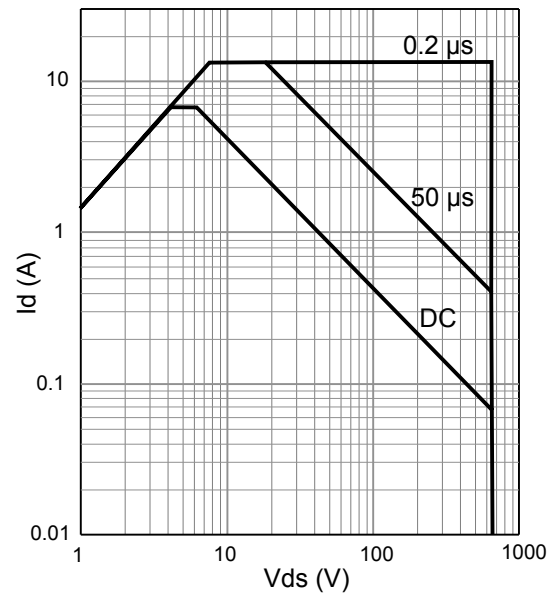
Figure 20. Safe Operating Area (HS) at T_J=25^\circ\text{C}
