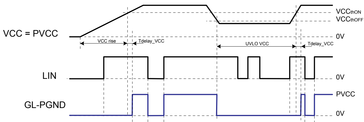
Figure 26. VCC UVLO and Low Side
