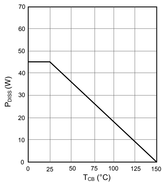
Figure 24. HS Derating curve
