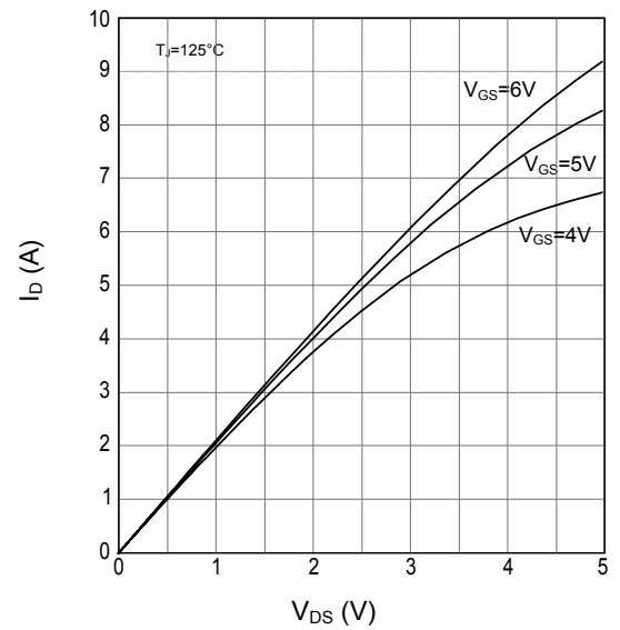
Figure 7. Typ I_{D\_HS} vs. V_{DS} at T_J=125^\circ\text{C}
