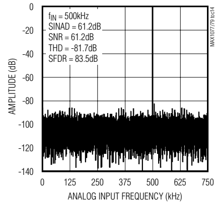
FFT PLOT (MAX1077)
