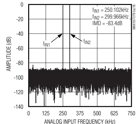
TWO-TONE IMD PLOT (MAX1079)
