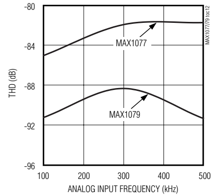
THD vs. INPUT FREQUENCY
