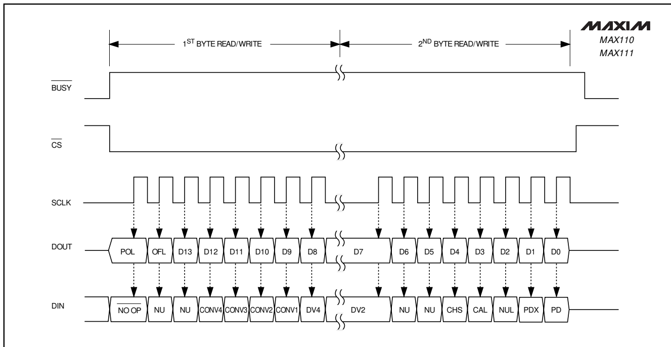
Figure 8a. SPI/MICROWIRE-Interface Timing
