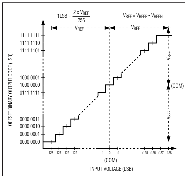
Figure 6. Transfer Function
