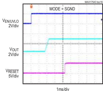
5V OUTPUT, PWM MODE SOFT-START WITH 2.5V PREBIAS, FIGURE 4a CIRCUIT
