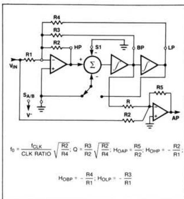
Figure 16. Mode 4a: 2nd-Order Filter Providing Highpass, Bandpass, Lowpass, Allpass
