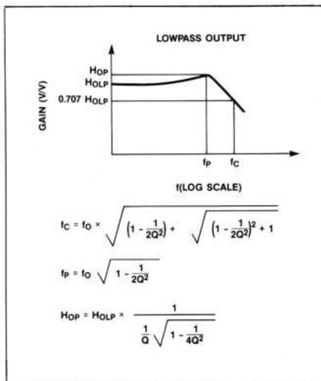
Figure 3. Lowpass Response
