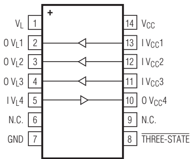
TSSOP-14 TOP VIEW
