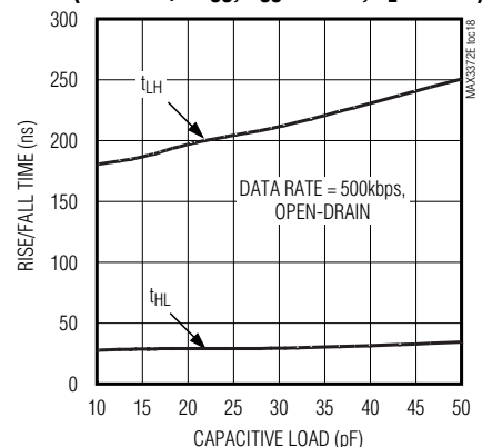
RISE/FALL TIME vs. CAPACITIVE LOAD (DRIVING I/O V_{CC} , V_{CC} = +3.3\text{V} , V_L = +1.8\text{V} )
