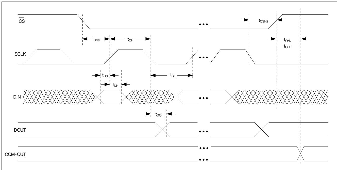
Figure 1. Timing Diagram
