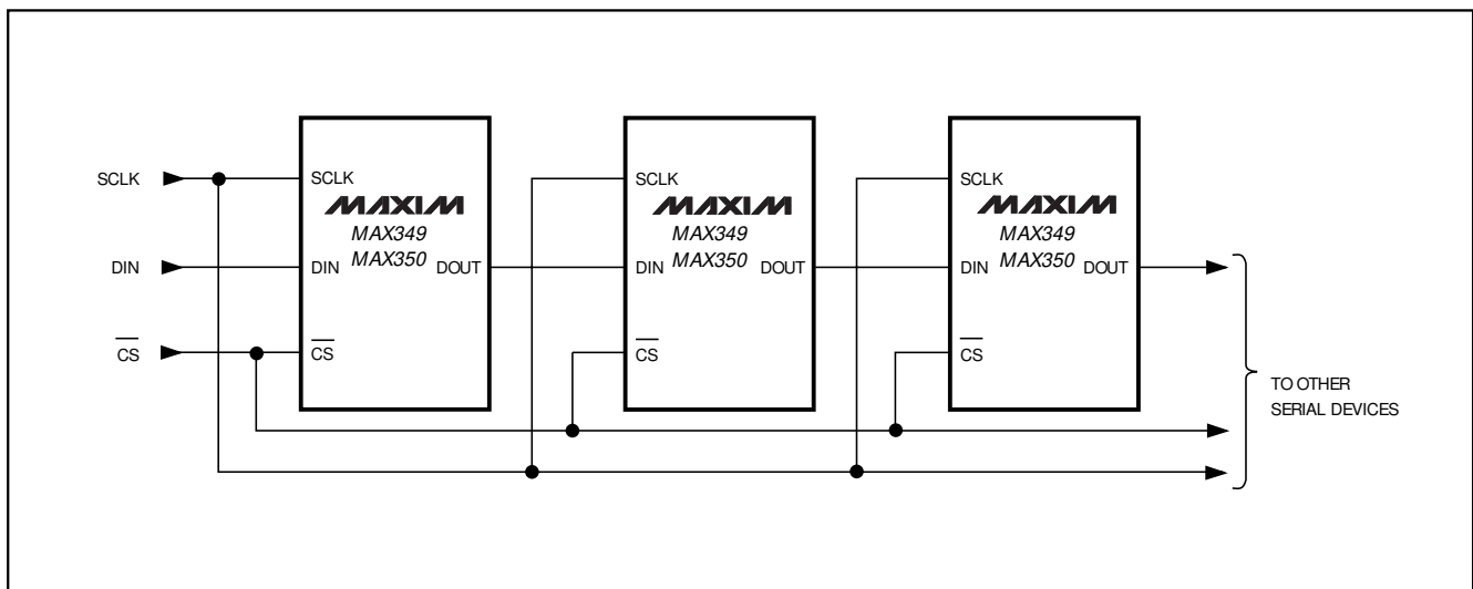
Figure 5. Daisy-Chained Connection
