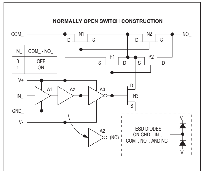
Figure 1. T-Switch Construction
