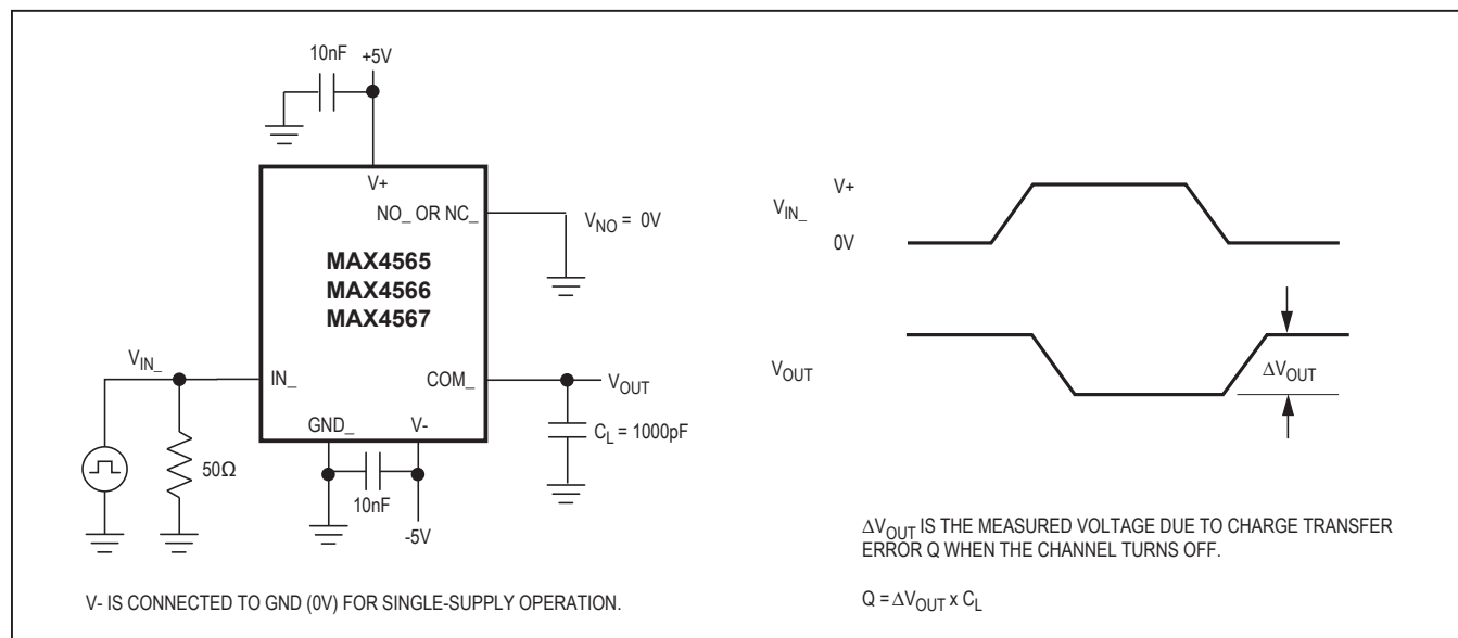
Figure 5. Charge Injection
