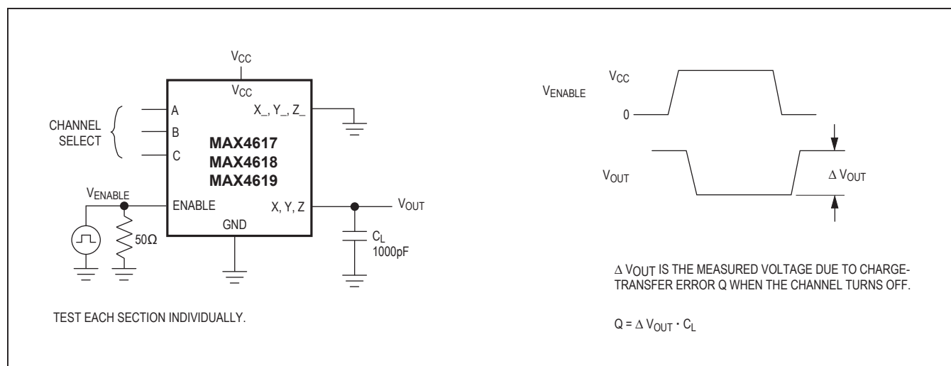
Figure 5. Charge Injection
