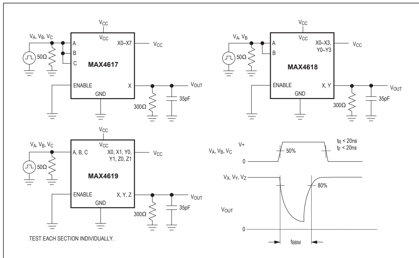
Figure 4. Break-Before-Make Interval
