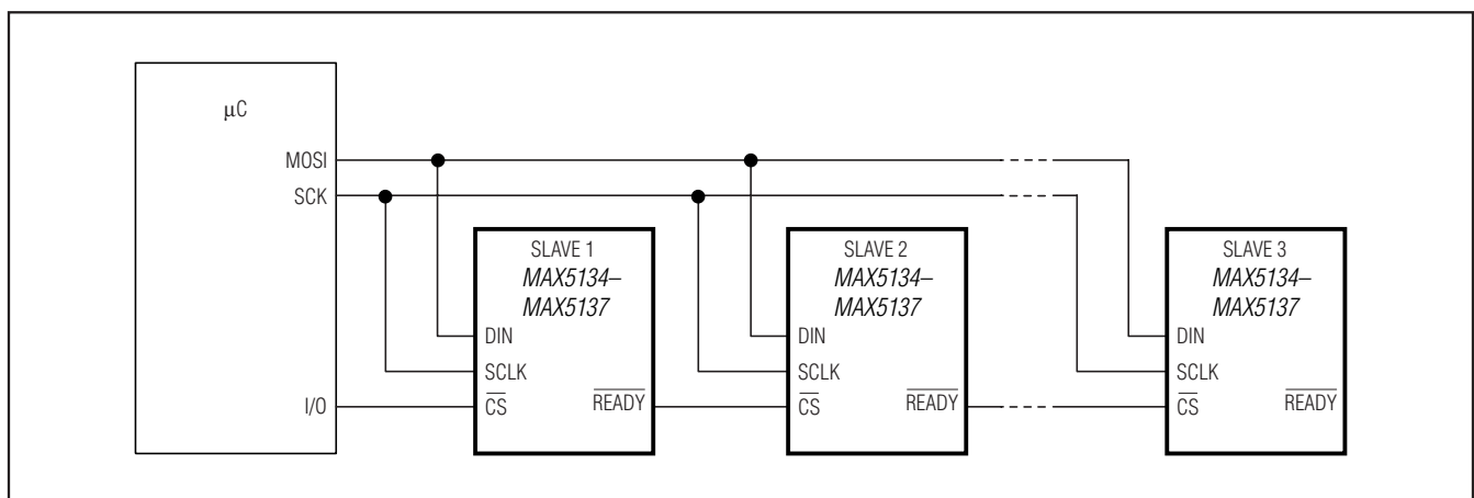
Figure 5. Daisy-Chain Configuration
