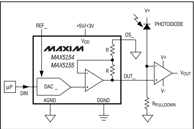
Figure 13. Digital Calibration
