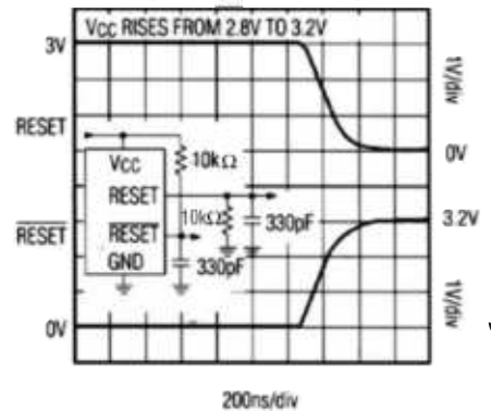
RESET, RESET RISE AND FALL TIMES (RESET DEASSERTED)
