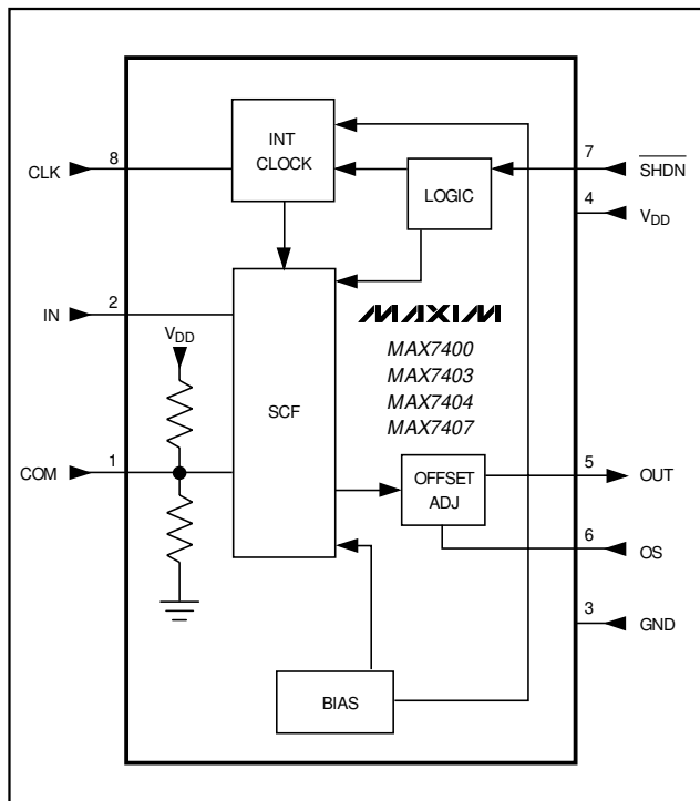
Figure 1. Functional Diagram
