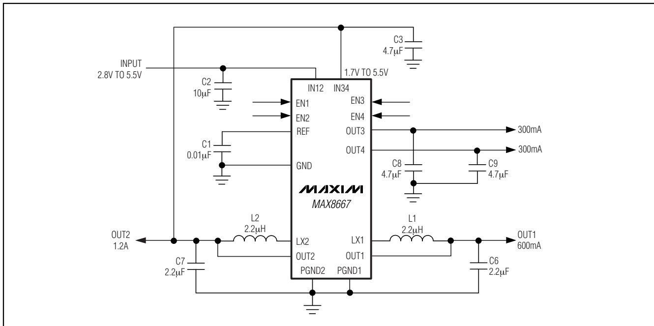
Figure 3. MAX8667 Typical Application Circuit
