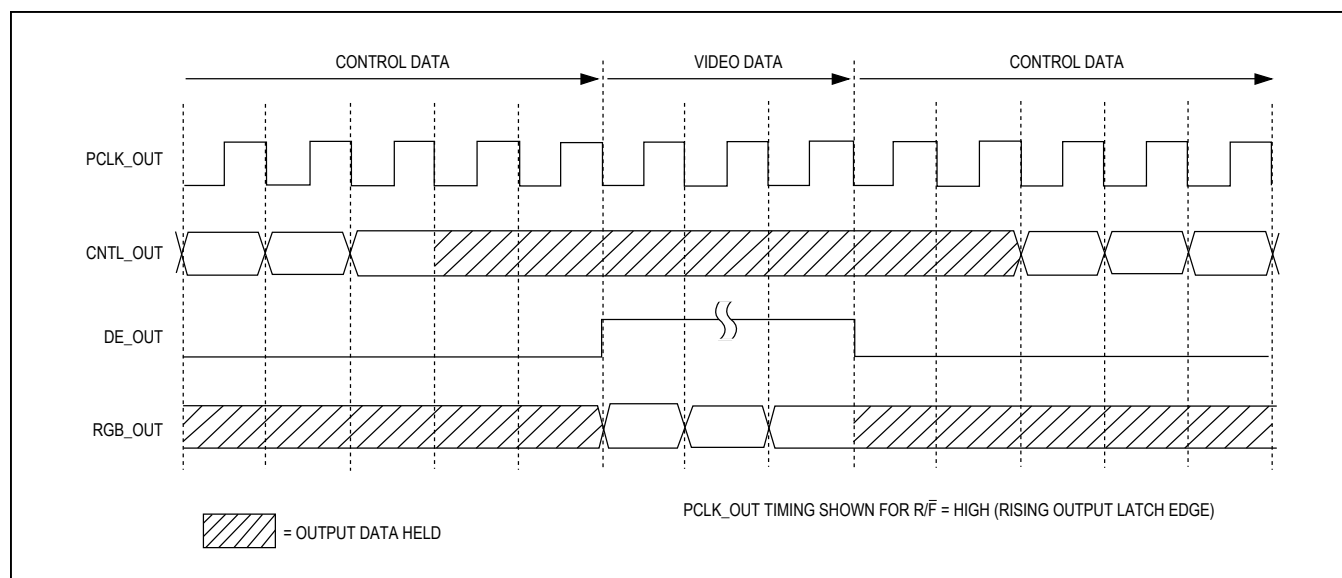
Figure 18. Output Timing
