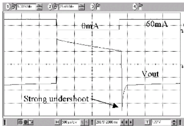
Figure 10. Without Load Transient Improvement
