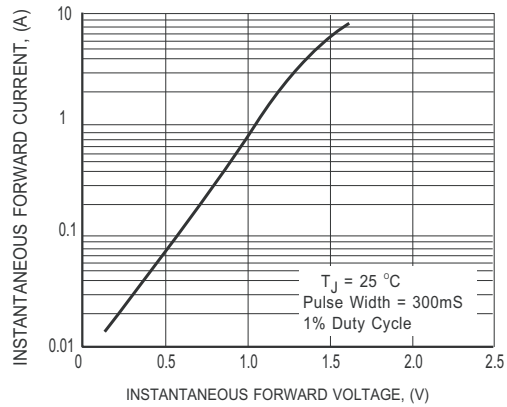
FIG.2 MAXIMUMN INSTANTANEOUS FORWARD CHARACTERISTICS
