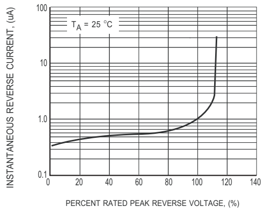
FIG.3 MAXIMUMN REVERSE CHARACTERISTICS
