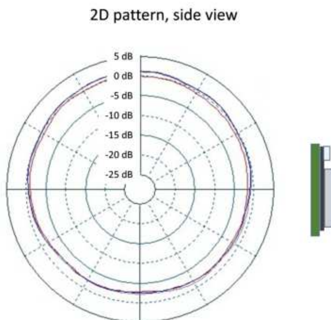
Figure 6.5. Typical 2D Radiation Pattern – Side View
