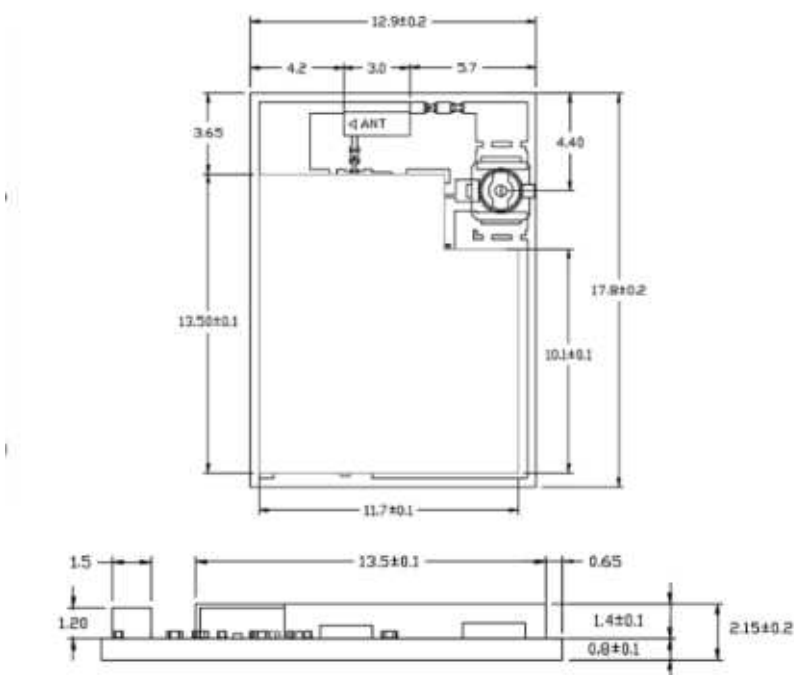
Figure 9.1. MGM13P with Antenna - Top and Side View
