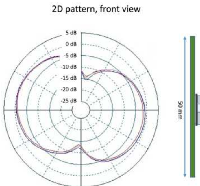
Figure 6.4. Typical 2D Radiation Pattern – Front View
