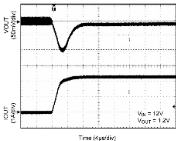
Transient Response
