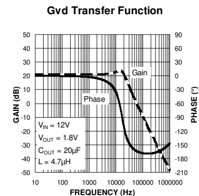
Figure 14. Gvd Transfer Function
