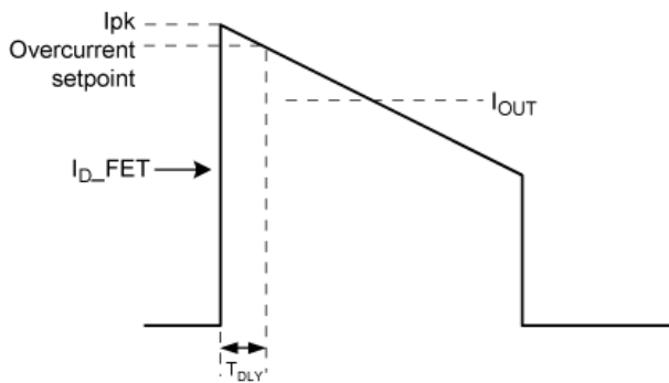
Figure 10. Overcurrent Waveform
