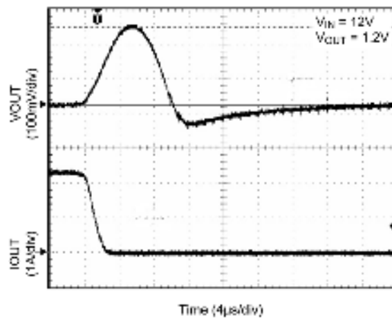
Transient Response
