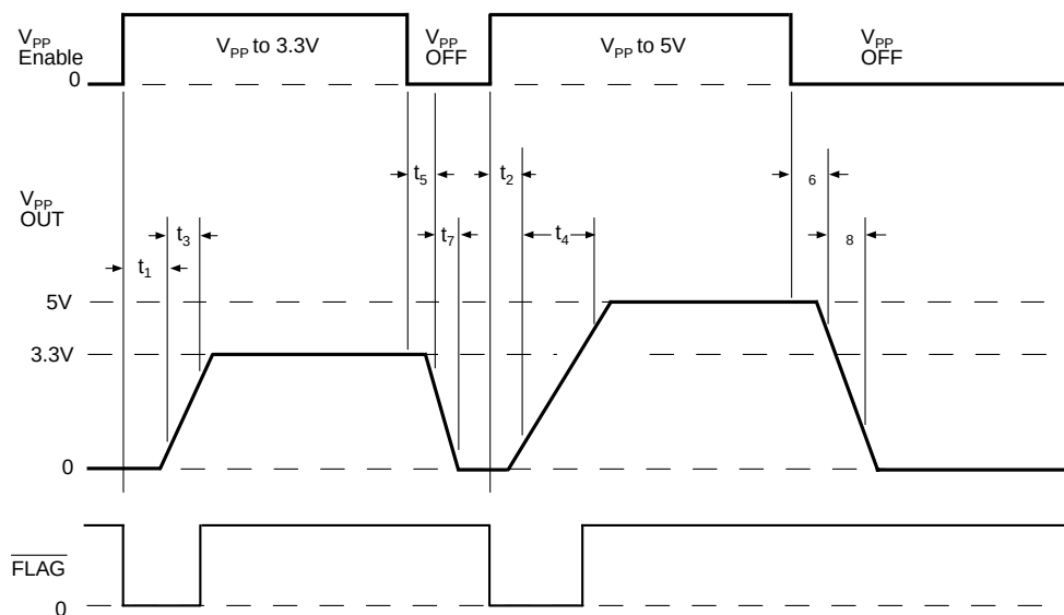
pp Timing Diagram
