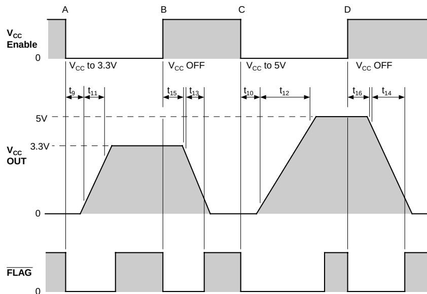
V_{CC} Timing Diagram
