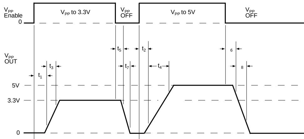
Figure 1. V_{PP} Timing Diagram
