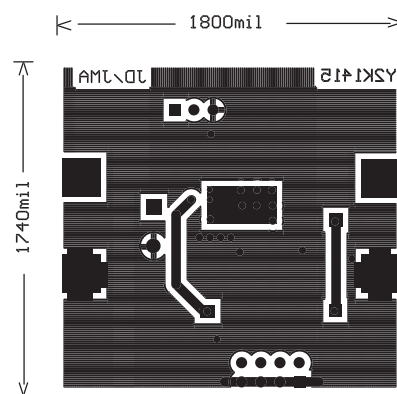
Figure 6e. Bottom-Side Copper
