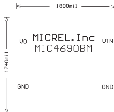
Figure 6d. Bottom-Side Silk Screen
