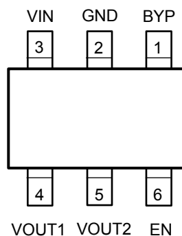
TSOT-23-6 (D6) Top View
