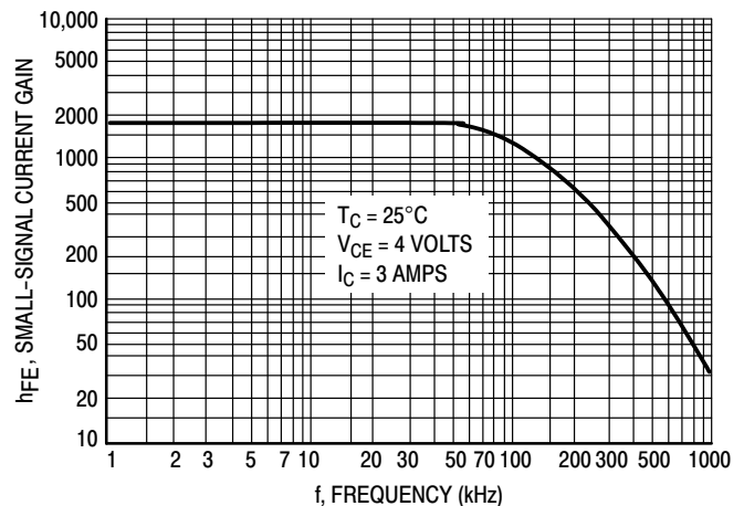
Figure 7. Typical Small-Signal Current Gain
