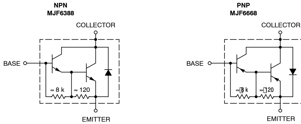
Figure 1. Darlington Schematic
