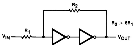
Figure 4. Schmitt Trigger
