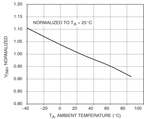
Figure 9. Inhibit Voltage vs. Temperature
