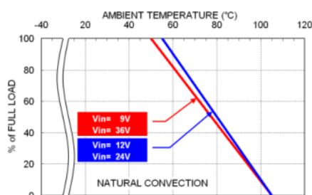
MPM20-24S□□W Derating Curve
