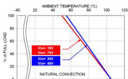
MPM20-48S□□W Derating Curve
