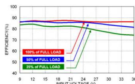
MPM20-24S05W Efficiency vs. Input Voltage
