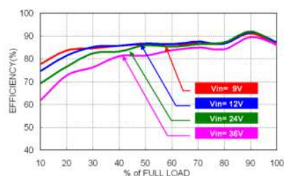
MPM20-24S05W Efficiency vs. Output Load
