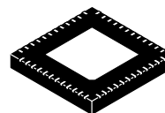
QFN48 7x7, 0.5P CASE 485EP
