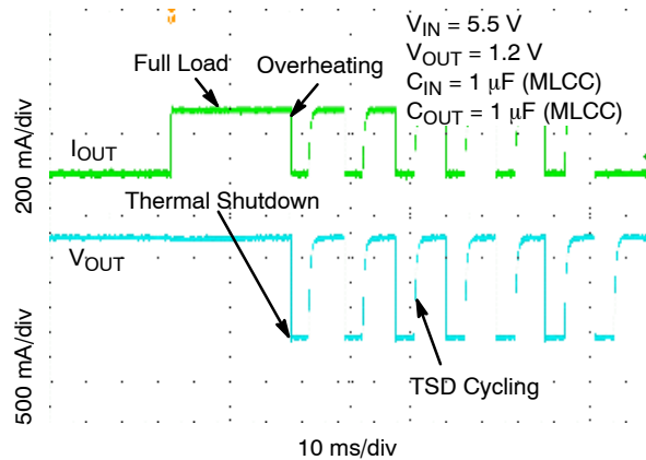
Figure 44. Short-Circuit and Thermal Shutdown
