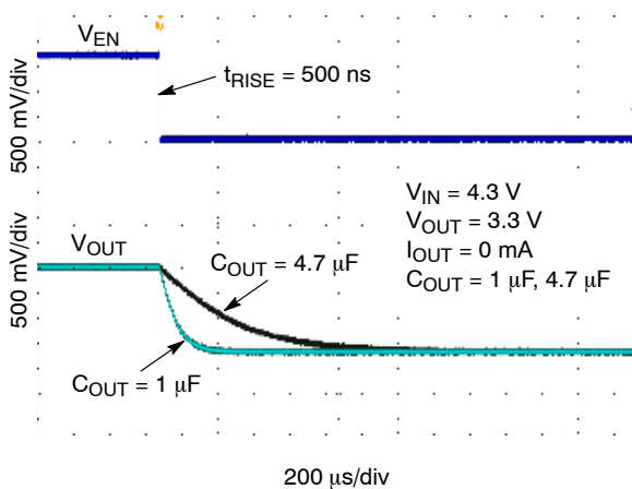
Figure 52. Enable Turn-Off – V_{OUT} = 1.0 V
