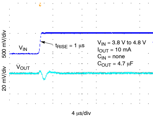
Figure 38. Line Transient Response– Rising Edge, V_{OUT} = 3.3 \text{ V} , I_{OUT} = 10 \text{ mA} , C_{OUT} = 4.7 \mu\text{F}
