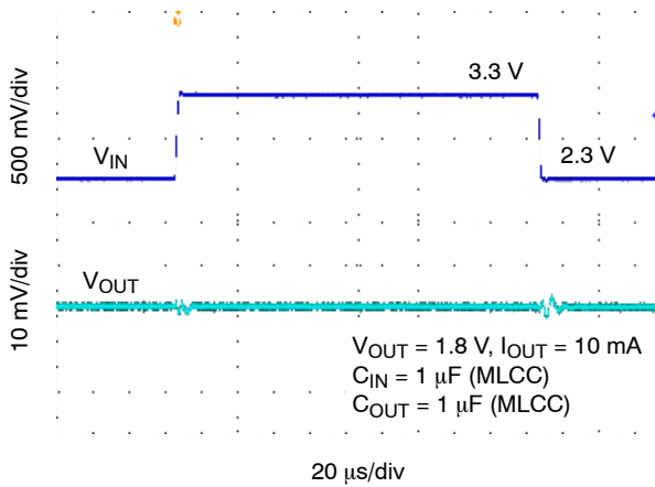
Figure 40. Line Transient Response – V_{OUT} = 1.8 V
