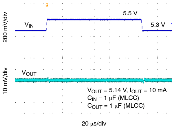
Figure 42. Line Transient Response – V_{OUT} = 5.14 V
