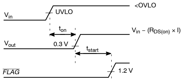
Figure 3. Startup
