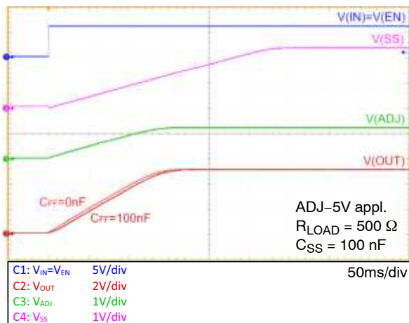
Figure 51. Startup by V_{IN} (ADJ=5V, C_{SS} = 100 nF)
