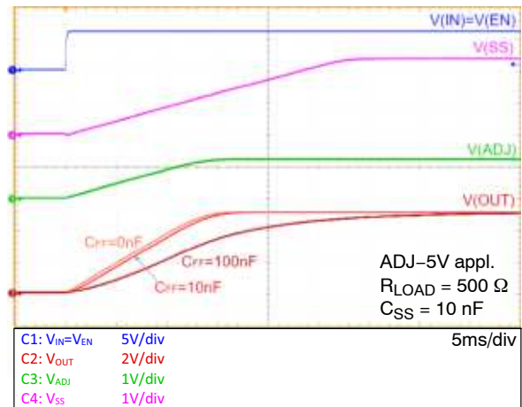
Figure 50. Startup by V_{IN} (ADJ=5V, C_{SS} = 10 nF)
