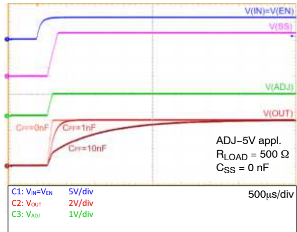
Figure 48. Startup by V_{IN} (ADJ=5V, C_{SS} = 0 nF)
