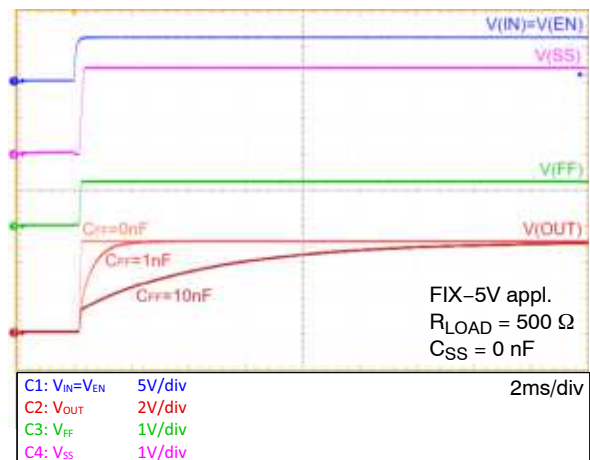
Figure 52. Startup by V_{IN} (FIX-5 V, C_{SS} = 0 nF)
