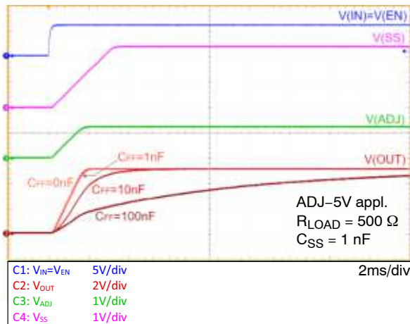
Figure 49. Startup by V_{IN} (ADJ=5V, C_{SS} = 1 nF)
