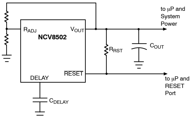
Figure 13. Adjustable \overline{\text{RESET}}
