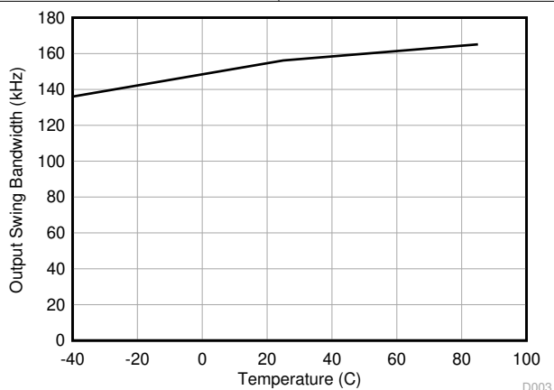
Figure 5-3. Output Swing Bandwidth vs Temperature at V_{CC} = \pm 10\text{ V}
