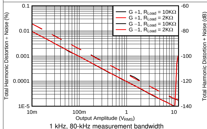
Figure 11. THD+N vs Output Amplitude
