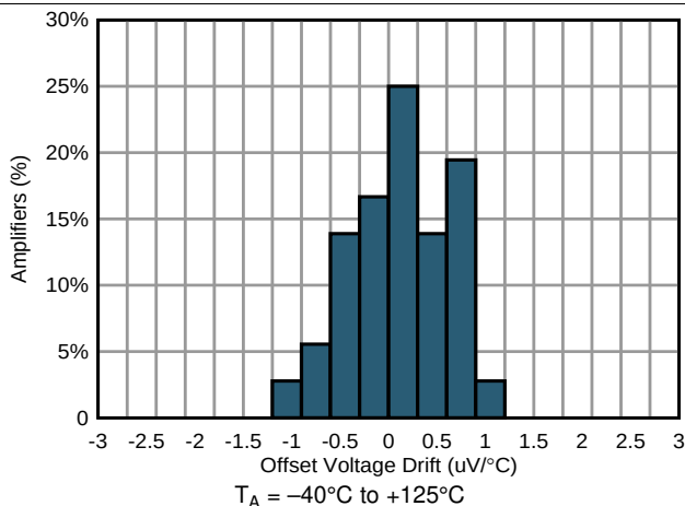
Figure 7. Offset Voltage Drift
