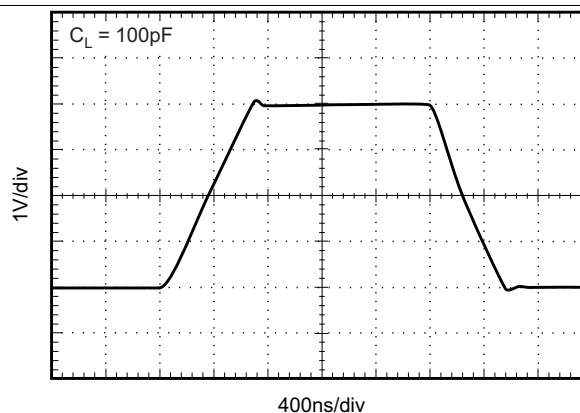
Figure 18. Large-Signal Step Response
