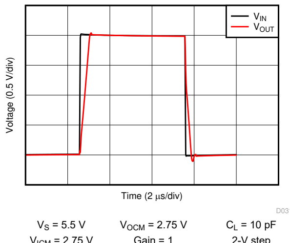
Figure 7-32. Large Signal Step Response
