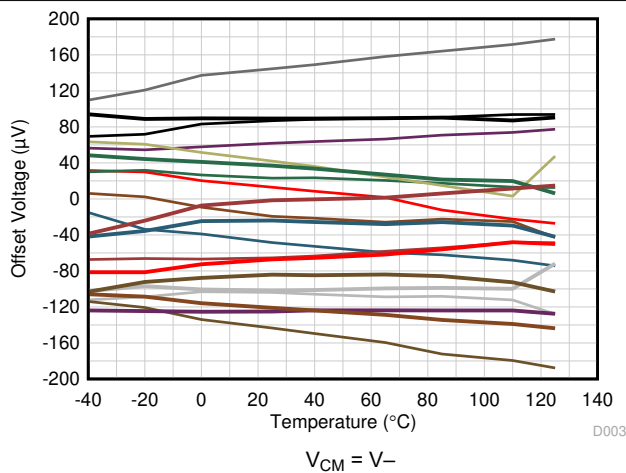
Figure 7-41. Offset Voltage vs Temperature (PMOS Input Pair)
