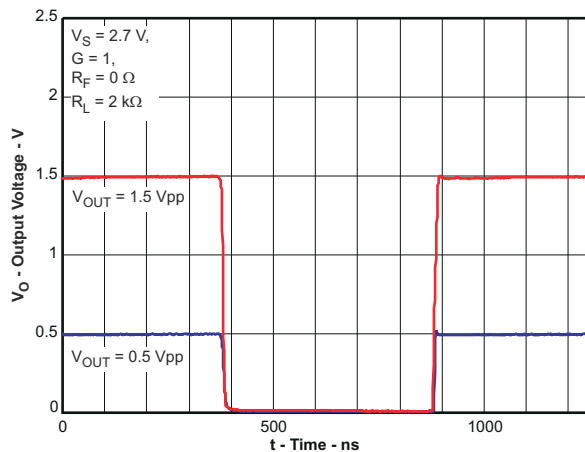
Figure 7-3. Noninverting Pulse Response
