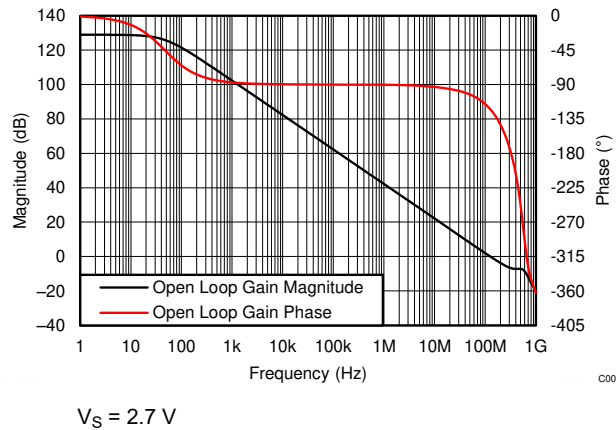
Figure 7-15. Open Loop Gain vs Frequency
