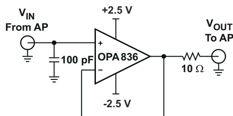
Figure 9-11. OPA836 Audio Precision Analyzer Test Circuit
