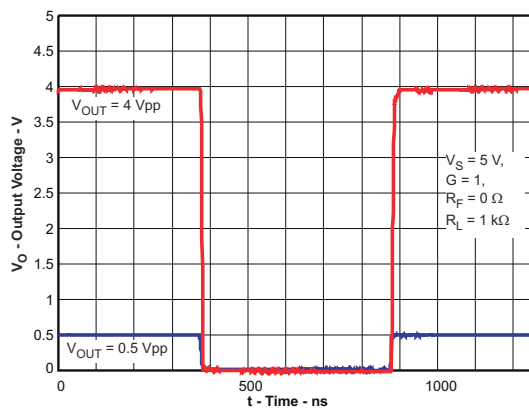
Figure 7-29. Noninverting Pulse Response
