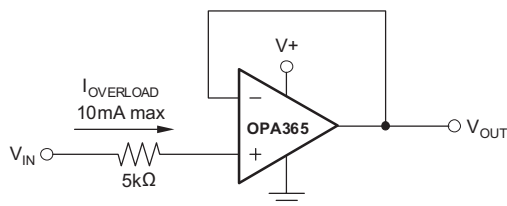
Figure 4. Input Current Protection
