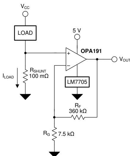
Figure 9-1. OPA191 in a Low-Side, Current-Sensing Application
