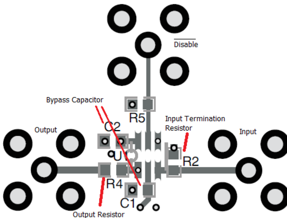
Figure 7-12. SBOS293 Layout
