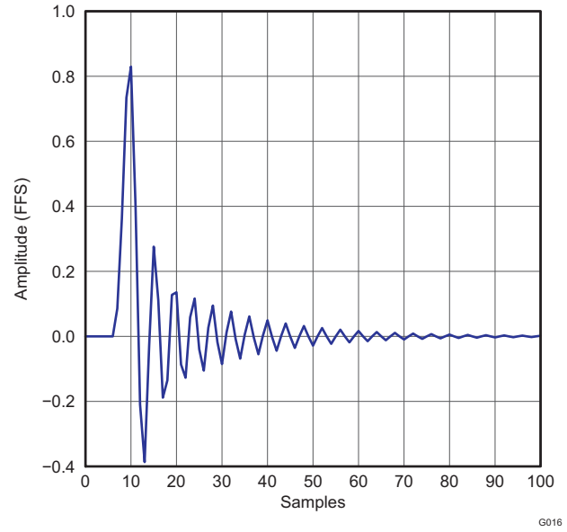
Figure 40. Low latency x2 Interpolation Filter Impulse Response
