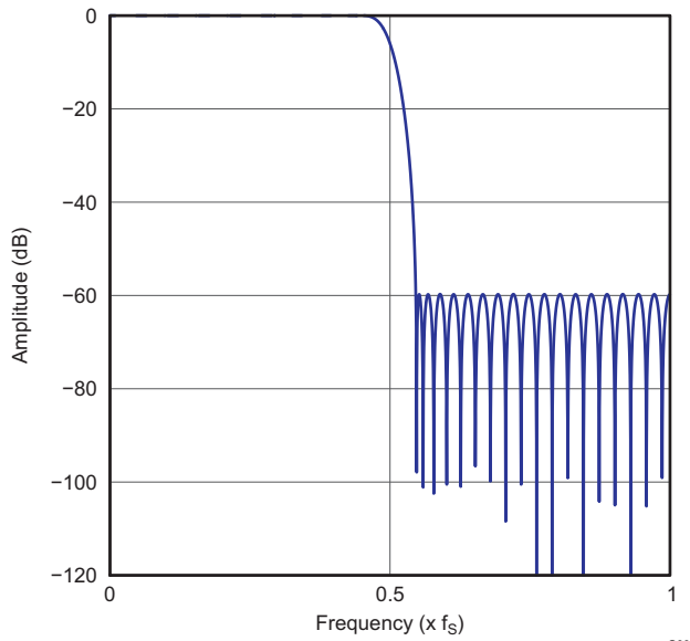
Figure 30. Normal x2 Interpolation Filter Frequency Response
