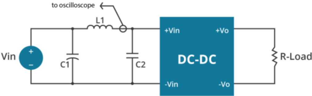
Figure 1 Measuring Input Ripple Current
