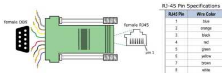
Figure B-10. Female DB-9 to RJ-45 Adapter and pinouts
