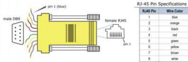
Figure B-09. Male DB-9 to RJ-45 Adapter and pinouts
