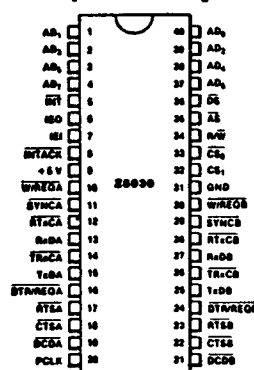
DIP Pin Assignments, 200030
