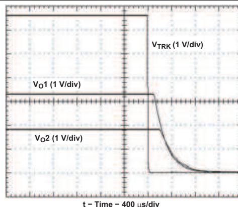
Figure 35. Simultaneous Power Down With Auto-Track Control
