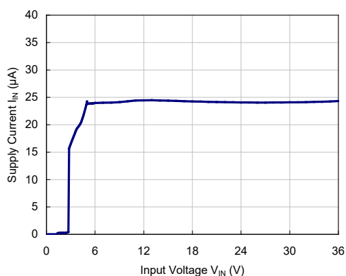
VR=5.0V
